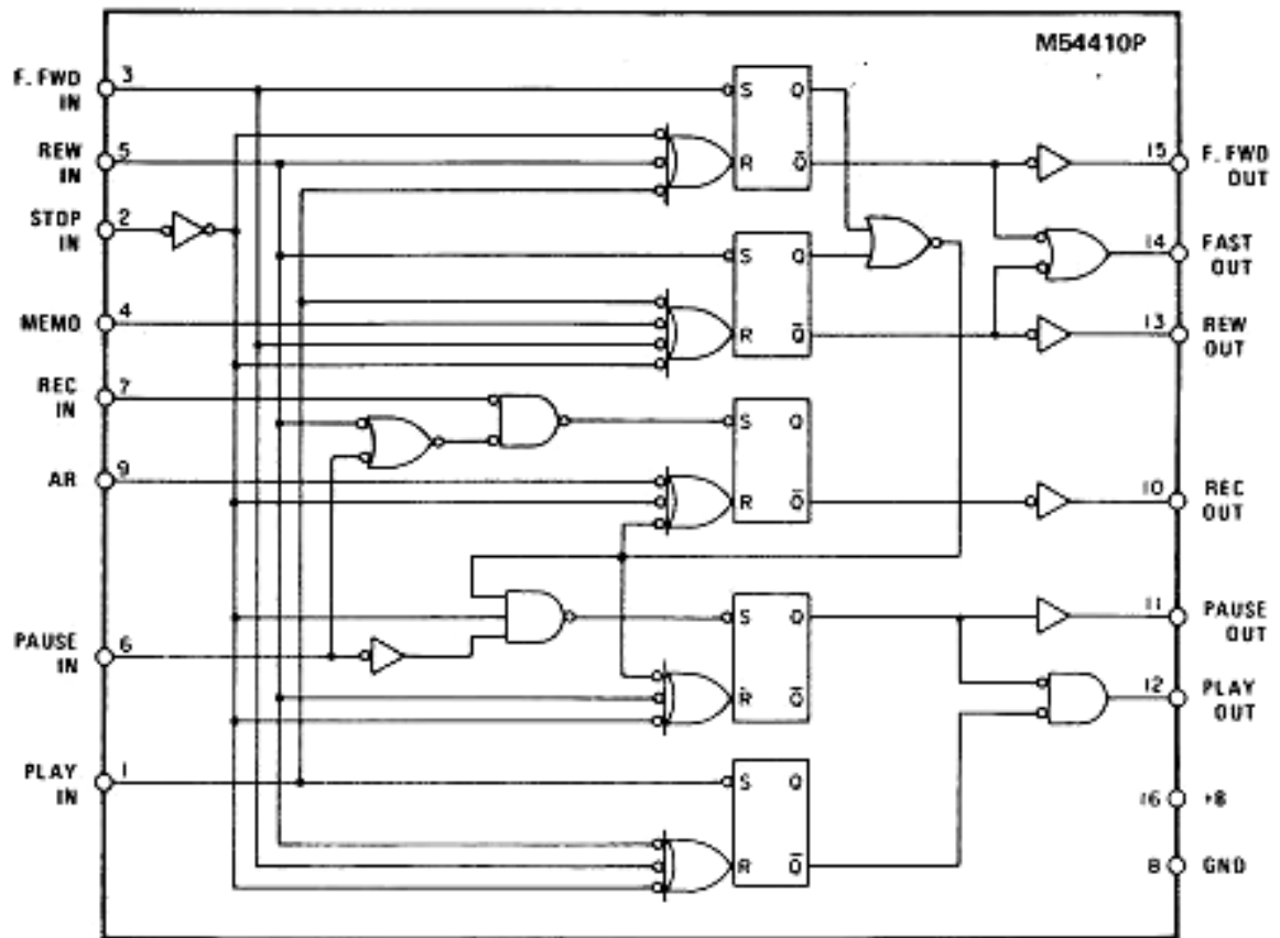
Fig. 1-2. Block Diagram
