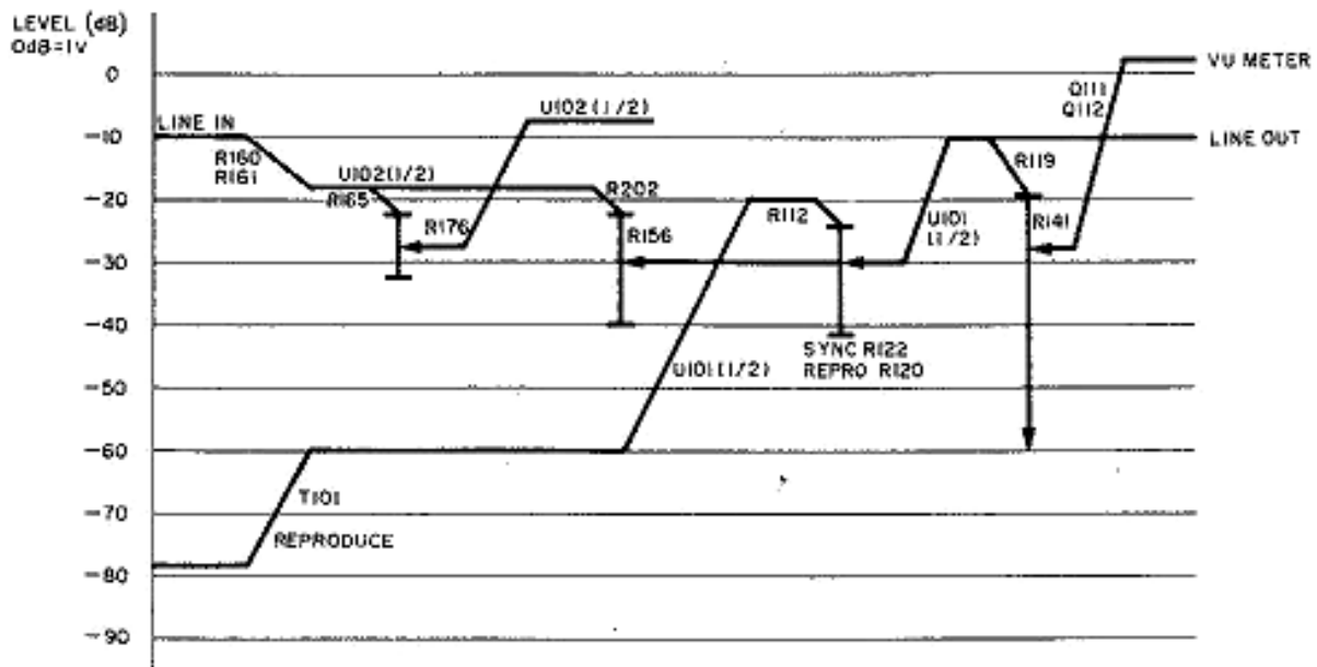
Fig. 1-17 Level Diagram
