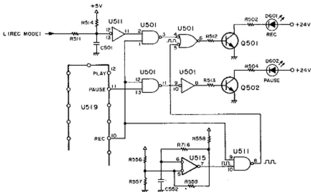
Fig. 1-13. Display Circuit
